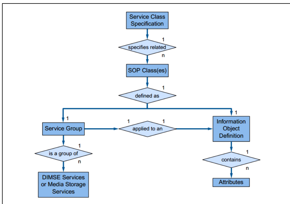
Abbildung 9: DICOM Information Model
